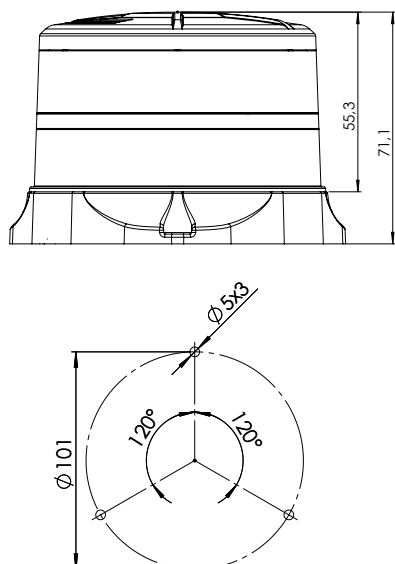
Surface mounting
