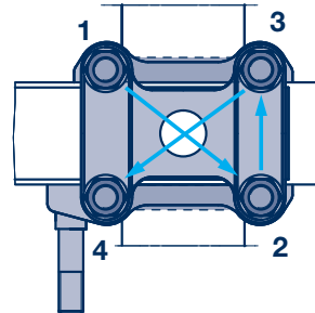
Spring U-bolt next to the axle beam
