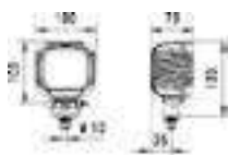
S 3000 LED
